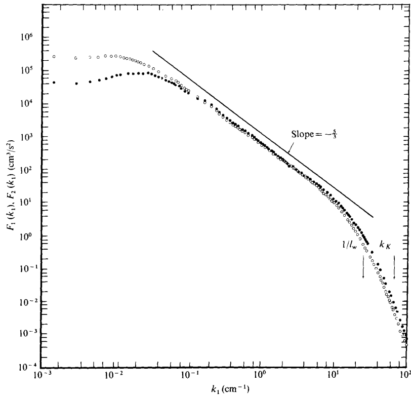
Figure 4.2: An experimentally-measured power spectrum for turbulence generated by an air jet (Champagne, 1978). The x axis is the wavenumber, and the open and filled points show the velocity power spectrum for the velocity components parallel and transverse to the stream, respectively.
