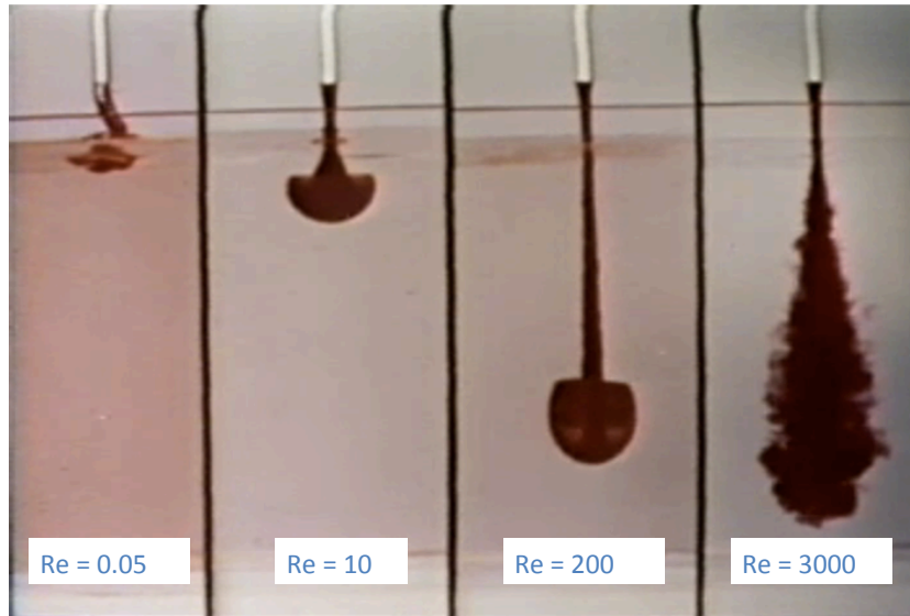
Figure 4.1: Flows at varying Reynolds number Re . In each panel, a fluid that has been dyed red is injected from the top into the clear fluid on the bottom. The fluids are a glycerin-water mixture, for which the viscosity can be changed by altering the glycerin to water ratio. By changing the viscosity and the injection speed, it is possible to alter the Reynolds number of the injected flow. The frames show how the flow develops as the Reynolds number is varied. This image is a still from the National Committee for Fluid Mechanics Film Series (Taylor, 1964), which, once you get past the distinctly 1960s production values, are a wonderful resource for everything related to fluids.
