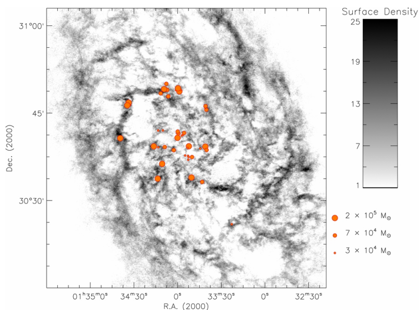
Figure 1.6: Map of H I in M33 (grayscale), with giant molecular clouds detected in CO(1 → 0) overlaid (circles, sized by GMC mass) (Imara et al., 2011).
