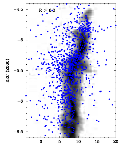
Figure 11.4: Measured distributions of ^{13}\text{CO} (grayscale) and young stellar objects (blue points) in velocity ( x axis) and position on the sky in one dimension ( y axis) for the Orion Nebula Cluster.
