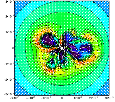
Figure 16.2: Results from a simulation of magnetized rotating collapse including the effects of ion-neutral drift and Ohmic dissipation (Krasnopolsky et al., 2012). Lengths on the axes are in units of cm. Colors and contours show the density in the equatorial plane, on a logarithmic scale from 10^{-16.5} to 10^{-12.5} \text{g cm}^{-3} . Arrows show velocity vectors.
