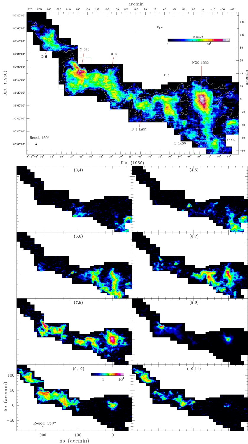
Figure 1.8: Map of the Perseus cloud in ^{13}\text{CO}(2 \rightarrow 1) from Sun et al. (2006). The top panel shows the emission integrated over all velocities, while the bottom panel shows maps integrated over different velocity channels. In each sub-panel in the bottom, the numbers at the top indicate the velocity range (in \text{km s}^{-1} ) of the emission shown.
