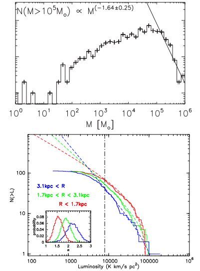
Figure 8.1: Two measurements of the GMC mass spectrum. The top panel shows the mass spectrum for the inner Milky Way determined from ^{13}\text{CO} measurements by Roman-Duval et al. (2010); the sample is complete at masses above \sim 10^5 M_\odot . The bottom panel shows the mass spectrum in M33, as determined by Gratier et al. (2012) using ^{12}\text{CO} . Note that these are cumulative distributions in luminosity, whereas the top panel shows a differential distribution in mass. The three colors show three different galactocentric regions: the inner galaxy (red), the mid-disk (green), and the outer galaxy (blue).
