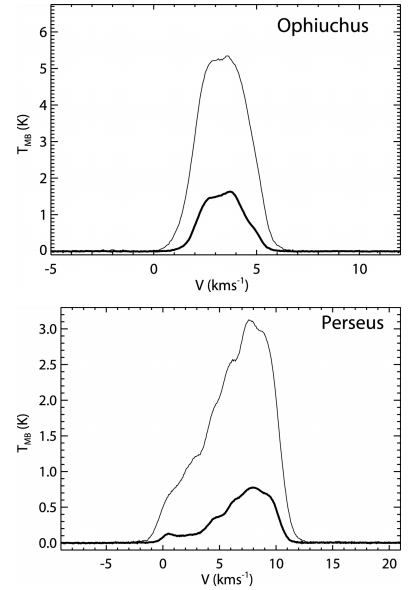
Figure 1.5: Position-integrated velocity distributions of ^{12}\text{CO} ( thin lines ) and ^{13}\text{CO} ( thick lines ) for the Ophiuchus and Perseus clouds, measured the COMPLETE survey (Ridge et al., 2006). The y axis shows the beam temperature.
