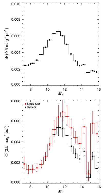
Figure 12.2: Luminosity function for Milky Way stars before (top) and after (bottom) bias correction (Bochanski et al., 2010).
