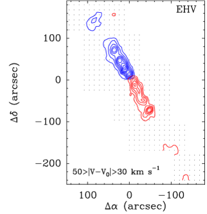
Figure 2.1: An integrated intensity map in \text{CO}(2 \rightarrow 1) , showing material at velocities between \pm 30 - 50 \text{ km s}^{-1} (blue and red contours, respectively) relative to the mean (Tafalla et al., 2004). Contours are spaced at intensities of 1 \text{ K km s}^{-1} . The outflow shown is in the Taurus star-forming region.
