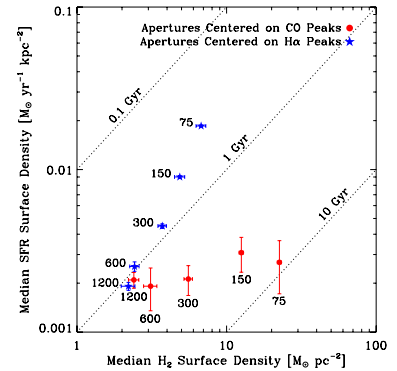
Figure 9.8: Kennicutt-Schmidt relation on different size scales. The points show the median surface densities of gas and star formation, using apertures of 75 – 1200 pc in size, centered in CO peaks (red) and \text{H}\alpha peaks (blue). Dotted lines of slope unity are lines of constant t_{\text{dep}} = \Sigma_{\text{SFR}} / \Sigma_{\text{mol}} , with the number indicating the depletion time.
