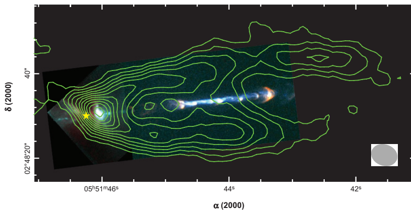
Figure 15.6: Color shows an HST image of the jet HH111. The green contours superimposed show an outflow detected as emission in the CO J = 1 \rightarrow 0 line at a velocity of 6 \text{ km s}^{-1} relative to the bulk of the material in the region. The yellow star marks the position of the driving source. The outflow is \approx 0.2 \text{ pc} long. (McKee & Ostriker, 2007).
