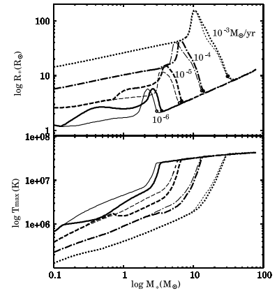
Figure 18.2: Radius versus mass (top panel) and maximum temperature versus mass (bottom panel) for protostars accreting at different rates. The accretion rate is indicated by the line style, as illustrated in the top panel. For each accretion rate there are two lines, one thick and one thin. The thick line is for the observed Milky Way deuterium abundance, while the thin line is the result assuming zero deuterium abundance.
