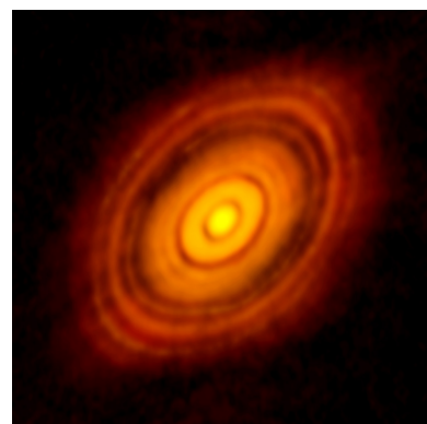
Figure 15.2: An ALMA image of the disk around the young star HL Tau. The image shows dust continuum emission. Image from https://public.nrao.edu/static/pr/planet-formation-alma.html .
