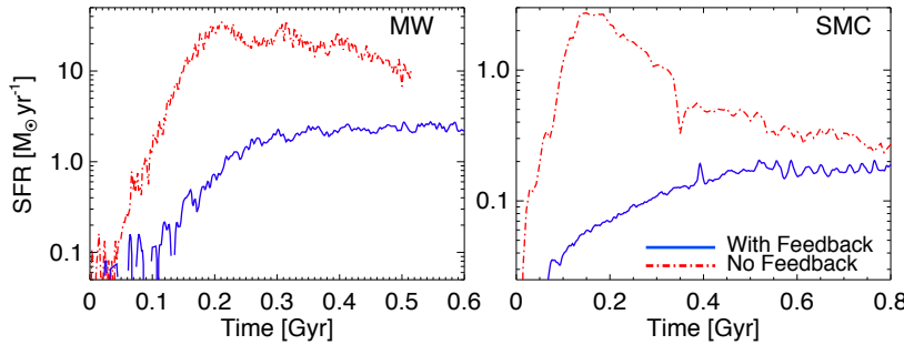
Figure 10.2: Star formation rates versus time measured in simulations of isolated galaxies performed with (blue) and without (red) a subgrid model for stellar feedback Hopkins et al. (2011). One simulation shown is for a galaxy with properties chosen to be similar to the Milky Way (left), and one is for a galaxy chosen to resemble the Small Magellanic Cloud (right).
