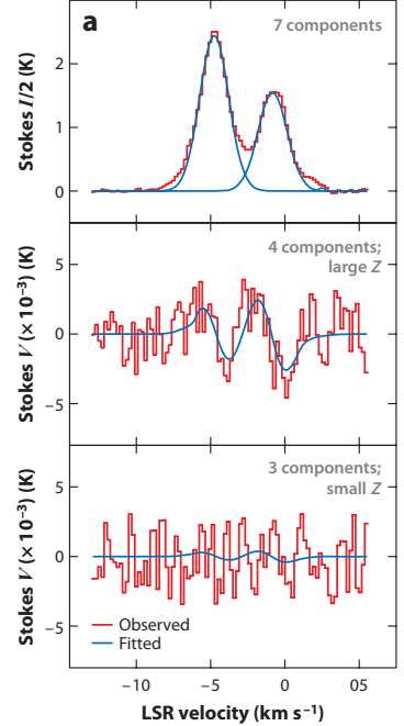
Figure 5.1: Sample Zeeman detection of an interstellar magnetic field using the CN line in the region DR21(OH) (Crutcher, 2012). The top panel shows the observed total intensity (Stokes I , red lines), which is well-fit by two different velocity components (blue lines). The CN molecule has 7 hyperfine components, of which 4 have a large Zeeman splitting and 3 have a small splitting. The middle panel shows the measured Stokes V (circularly polarized emission) for the sum of the 4 strong splitting components, while the bottom panel shows the corresponding measurement for the 3 weak components. The blue lines show the best fit, with the line of sight magnetic field as the fitting parameter.
