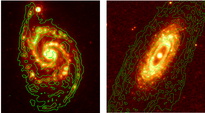
Figure 8.9: The galaxies NGC 5194 (left) and NGC 2841 (right), imaged in H I from THINGS and 24 \mu\text{m} from Spitzer (Tamburro et al., 2008).
