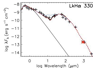
Figure 19.6: The spectral energy distribution of the star LkH \alpha 330 (Brown et al., 2008). Plus signs indicate measurements. The black line is a model for a stellar photosphere. The blue line is a model for a star with a disk going all the way to the central star, while the red line is a model in for a disk with a 40 AU hole in its center.
