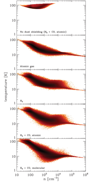
Figure 10.4: Density-temperature distributions measured in simulations with different treatments of ISM thermodynamics and chemistry Glover & Clark (2012). All simulations use identical initial conditions, but vary in how the gas heating and cooling rates are calculated. The top panel ignores dust shielding, but includes full chemistry and heating and cooling. The bottom panel includes all chemistry and cooling. The middle three panels turn off, respectively, \text{H}_2 formation, CO formation, and CO cooling. The tail of material proceeding to high density in some simulations is indicative of star formation.
