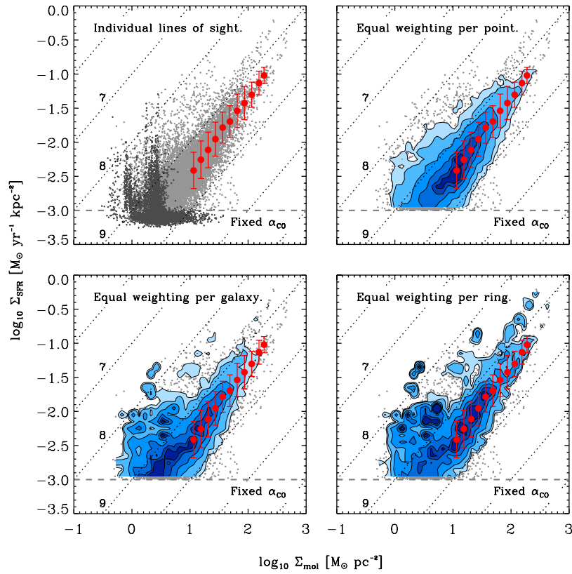
Figure 9.6: Kennicutt-Schmidt relation for \sim kpc-sized lines of sight through a sample of nearby galaxies (Leroy et al., 2013), computed with fixed CO-H 2 conversion factor. The four panels show points individual lines of sight (top left), contours with equal weighting per line of sight (top right), contours with equal weighting per galaxy (bottom left) and contours with equal weighting per azimuthal ring (bottom right). Dotted lines of slope unity are lines of constant t_{\text{dep}} = \Sigma_{\text{SFR}}/\Sigma_{\text{mol}} , with the number indicating the log of the depletion time in yr. Gray horizontal dashed lines mark the star formation rate sensitivity limit.
