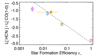
Figure 10.3: Ratio of HCN to CO luminosity computed from simulations of galaxies that are identical except for their subgrid model for the star formation rate in dense gas, parameterized by \epsilon_* Hopkins et al. (2013).
