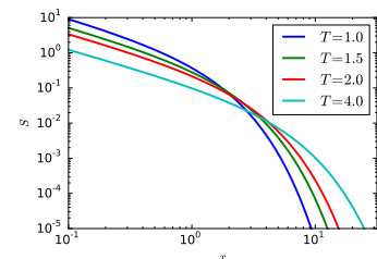
Figure A.5: S versus x at dimensionless times T = 1, 1.5, 2, and 4 .
