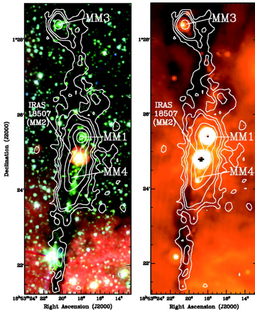
Figure 14.1: A typical infrared dark cloud (IRDC) (Rathborne et al., 2006). The left image shows Spitzer /IRAC (near-IR), where the cloud is seen in absorption against the galactic background, while the right image shows Spitzer /MIPS (mid-IR), where parts are seen in absorption and parts in emission. The white contours, which are the same in both panels, show mm continuum emission.
