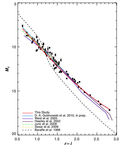
Figure 12.1: Color-magnitude diagram for stars with well-measured parallax distances Bochanski et al. (2010). The filters used are the SDSS r and i .
