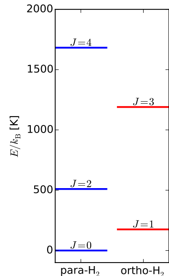
Figure 1.1: Level diagram for the rotational levels of para- and ortho- H_2 , showing the energy of each level. Level data are taken from http://www.gemini.edu/sciops/instruments/nir/wavecal/h2lines.dat .
