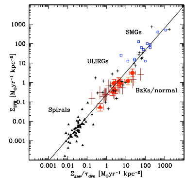
Figure 9.4: Kennicutt-Schmidt relation including an expanded high-redshift sample, now including orbital time Daddi et al. (2010). Points are the same as in Figure 9.3, except that points for which the orbital time \tau_{\text{dyn}} are unavailable have been omitted.
