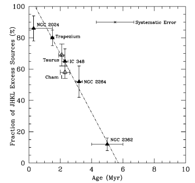
Figure 19.5: Fraction of stars that show near-infrared excess emission versus cluster age. The names of individual clusters are marked. Figure from Haisch et al. (2001).
