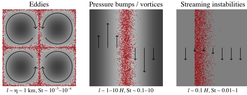
Figure 20.1: Schematic diagram of three mechanisms to concentrate particles in a protoplanetary disk. The left panel shows how small-scale turbulent eddies expel particles to their outskirts. The middle panel shows how zonal flows associated with large-scale pressure bumps concentrate particles. The right panel shows concentration by streaming instabilities. In each panel, black arrows show the velocity field, and the caption indicates the characteristic length scale of the structures shown, where H is the disk scale height.
