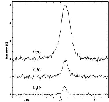
Figure 11.3: Velocity distributions measured toward a nearby protostellar core using three different molecular line tracers, as indicated. The transitions ^{13}\text{CO} , \text{C}^{18}\text{O} , and \text{N}_2\text{H}^+ should be roughly ordered from lowest to highest in terms of the density of gas that produces them.
