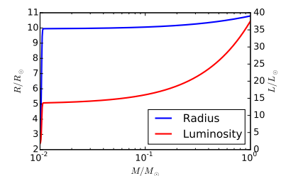
Figure A.6: Radius (blue) and luminosity (red) for the simple protostellar evolution model.
