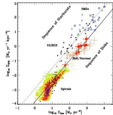
Figure 9.3: Kennicutt-Schmidt relation including an expanded high-redshift sample, with two proposed sequences (“disks” and “starbursts”) indicated Daddi et al. (2010). Points are integrated-galaxy measurements, while contours are spatially-resolved regions (see below).
