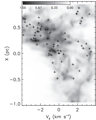
Figure 11.7: Distributions of ^{13}\text{CO} (grayscale) and young stellar objects (black crosses) in velocity ( x axis) and position on the sky in one dimension ( y axis) in a simulation of the Orion Nebula Cluster (Offner et al., 2009).
