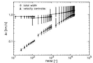
Figure 4.3: Linewidth versus size in the Polaris Flare Cloud obtained from CO observations (Ossenkopf & Mac Low, 2002). Diamonds show the total measured velocity width within apertures of the size indicated on the x axis, while triangles show the dispersion obtained by taking the centroid velocity in each pixel and measuring the dispersion of centroids. The three sets of points joined by lines represent measurements from three separate telescopes.
