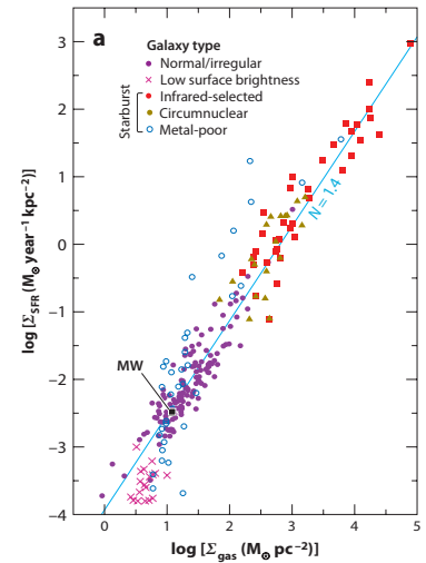
Figure 9.1: The observed collection between gas surface density \Sigma_{\text{gas}} and star formation surface density \Sigma_{\text{SFR}} , integrating over whole galaxies. Galaxy classes are as indicated in the legend. Taken from Kennicutt & Evans (2012).
