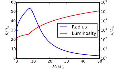
Figure A.7: Radius (blue) and luminosity (red) for the simple protostellar evolution model for a massive star.
