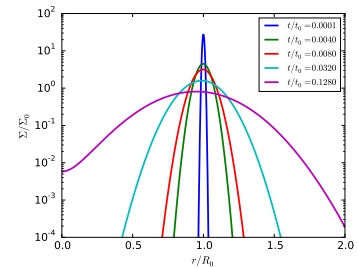
Figure 16.3: Analytic solution for the viscous ring of material with constant kinematic viscosity \nu . At time t = 0 , the column density distribution is \Sigma = \Sigma_0 \delta(r - R_0) . Colored lines show the surface density distribution at later dimensionless times, as indicated in the legend. The analytic solution shown is that of Pringle (1981).
