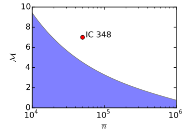
Figure A.4: Mach number \mathcal{M} versus mean density \bar{n} , separating the region where f(> x_0) < f_{\text{BD}} (shaded) from the region where f(> x_0) > f_{\text{BD}} . The red point shows the properties of IC 348.
