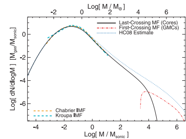
Figure 13.2: The IMF predicted by an analytic model of turbulent fragmentation by Hopkins (2012).
