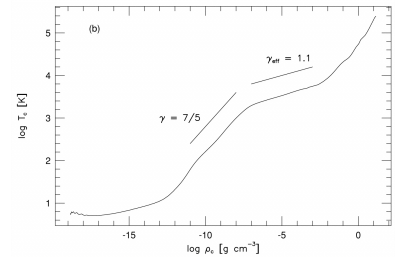
Figure 13.3: Temperature versus density found in a one-dimensional calculation of the collapse of a 1 M_{\odot} gas cloud, at the moment immediately before a central protostar forms (Masunaga & Inutsuka, 2000).
