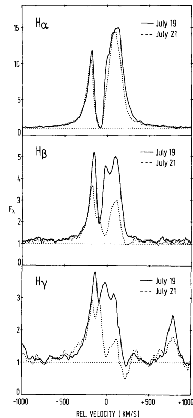
Figure 19.1: Observed line profiles for three Balmer lines from the T Tauri star S Cr A taken on two nights in July, 1983. Figure from Appenzeller & Mundt (1989).
