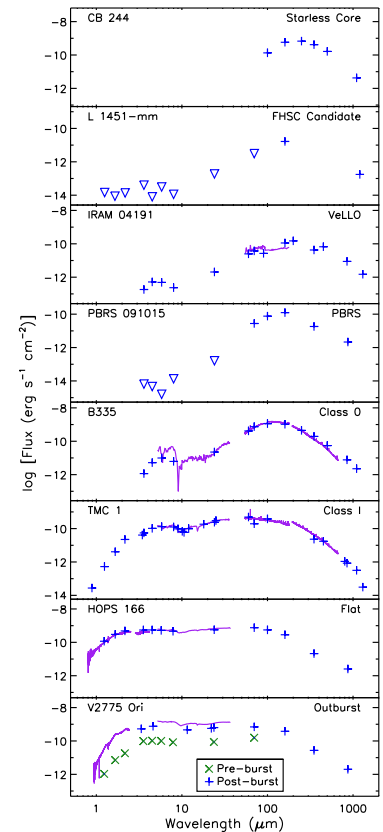
Figure 2.2: Sample spectral energy distributions (SEDs) of protostellar cores, together with the assigned class, as collected by Dunham et al. (2014).
