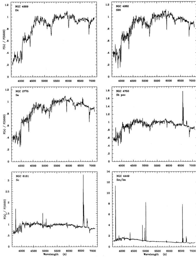
Figure 2.6: Example spectra of galaxies of varying Hubble type, from the atlas of Kennicutt (1992). In each panel, the galaxy name and Hubble type are listed.
