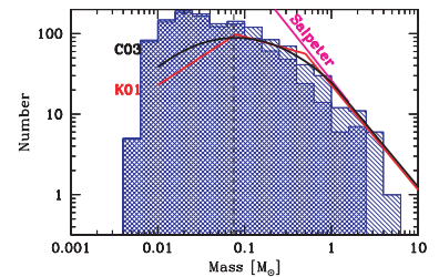
Figure 13.1: The IMF measured in a simulation of the collapse of a 500 M_{\odot} initially uniform density cloud (Bate, 2009a). The single-hatched histogram shows all objects in the simulation, while the double-hatched one shows objects that have stopped accreting.
