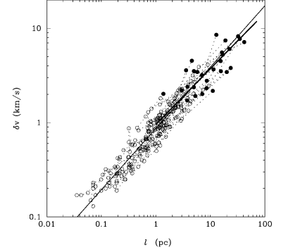
Figure 8.3: Measured correlation between GMC linewidth \delta v and size scale \ell for Milky Way clouds (Heyer & Brunt, 2004).
