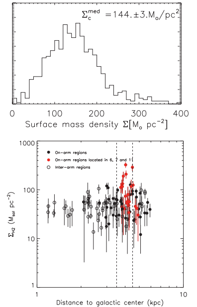
Figure 8.2: Two measurements of GMC surface densities. The top panel shows the distribution of surface densities for the inner Milky Way determined from ^{13}\text{CO} measurements by Roman-Duval et al. (2010). The bottom panel shows GMC surface density versus galactocentric radius in NGC 6946, measured from both ^{12}\text{CO} and ^{13}\text{CO} (Rebolledo et al., 2012).
