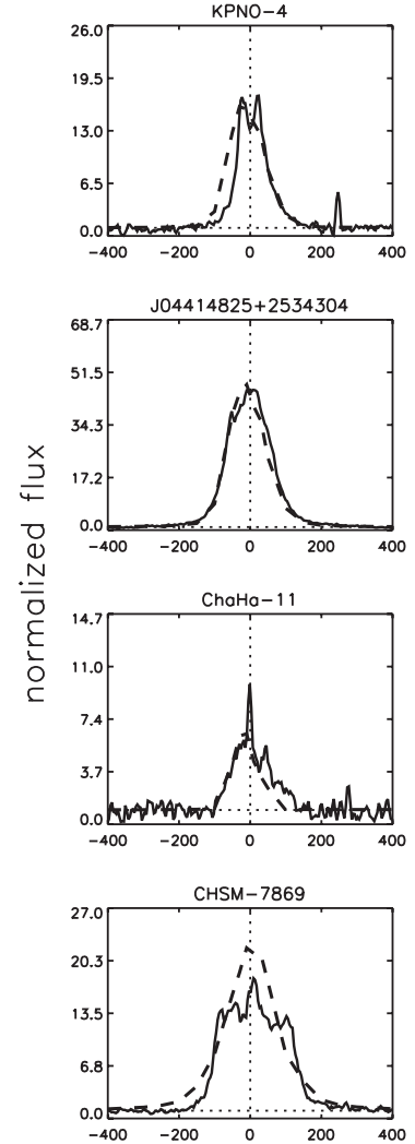
Figure 19.2: Comparisons between observed (solid) and model (dashed) H\alpha line profiles for a sample of T Tauri stars (Muzerolle et al., 2005). The x axis shows velocity in \text{km s}^{-1} . Each model curve is a fit in which the accretion rate is one of the free parameters.
