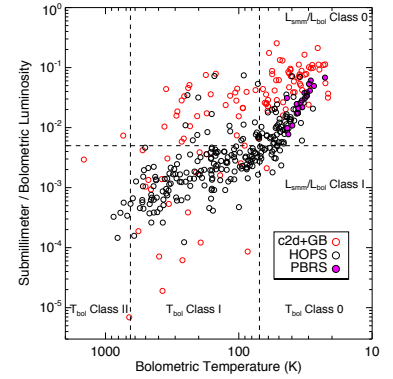
Figure 2.3: Bolometric temperatures of protostellar cores as compared to sub-mm to bolometric luminosity ratios (Dunham et al., 2014). The samples shown are from three different surveys as indicated in the legend.
