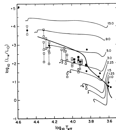
Figure 18.4: Thin lines show tracks taken by stars of varying masses (indicated by the annotation, in M_{\odot} ) in the theoretical HR diagram of luminosity versus effective temperature. Stars begin at the upper right of the tracks and evolve to the lower left; tracks end at the main sequence. The thick line crossing the tracks is the birthline, the point at which the stars stop accreting and become optically visible. Squares and circles represent the properties of observed young stars. Figure taken from Palla & Stahler (1990).
