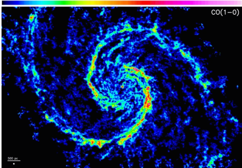
Figure 1.7: Map of CO(1 → 0) emission in M51, as measured by the PdBI Arcsecond Whirlpool Survey (PAWS) project (Schinnerer et al., 2013).
