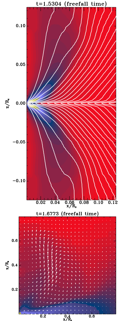
Figure 16.1: Results from a simulation of magnetized rotating collapse (Hennebelle & Fromang, 2008). The top panel shows the magnetic field structure; solid lines are poloidal magnetic field lines, while color indicates the azimuthally-averaged total magnetic field strength, on a scale from 0 – 3.5 mG. The bottom panel shows the density (color) and velocity (arrows) structure at a slightly later time in the simulation. The structure in the mid-plane is a non-rotating pseudo-disk.
