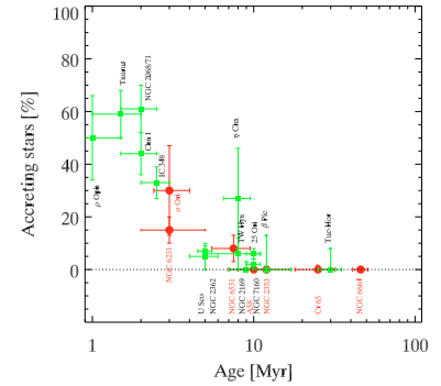
Figure 19.4: Fraction of stars that show evidence of accretion, as indicated by H\alpha line emission, for clusters of different ages (indicated on the x axis). The names of individual clusters are marked. Figure from Fedele et al. (2010).
