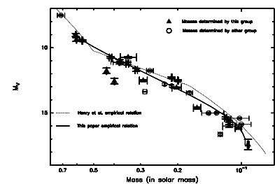
Figure 12.3: Empirically-measured mass-magnitude relationship in V band (Delfosse et al., 2000).
