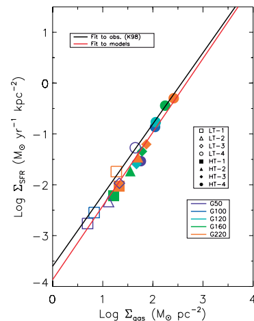
Figure 10.1: Relationship between gas surface density \Sigma_{\text{gas}} and star formation surface density \Sigma_{\text{SFR}} , measured from a series of simulations using no physics except hydrodynamics and gravity Li et al. (2005).
