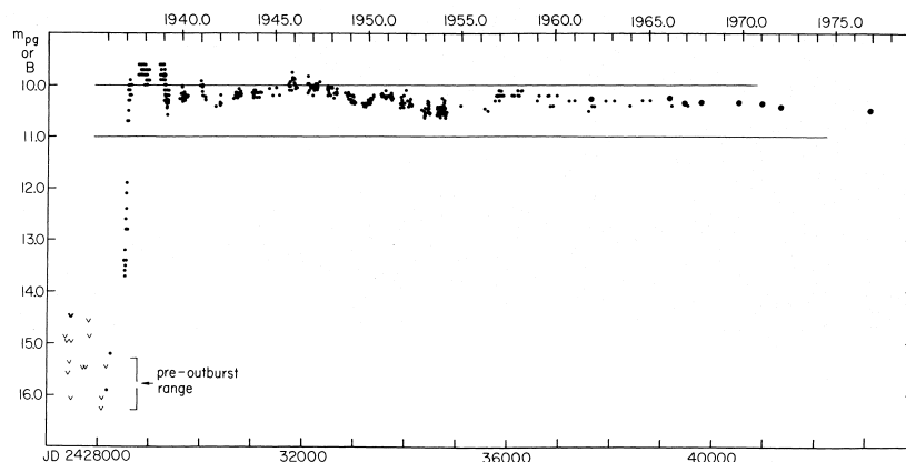
Figure 19.3: A light curve of the star FU Orionis, from the 1930s to 1970s (Herbig, 1977). The y axis shows the apparent magnitude in B band, or from photographic observations prior to filter standardization.
