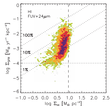
Figure 9.9: Kennicutt-Schmidt relation for H I gas in inner galaxies, averaged on \sim 750 pc scales Bigiel et al. (2008). Contours indicate the density of points.
