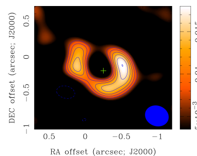
Figure 19.7: Dust continuum image of the disk around LkH \alpha 330, taken at 340 GHz by the SMA (Brown et al., 2008). Colors show the detected signal, and contours show the signal to noise ratio, starting from S/N of 3 and increasing by 1 thereafter. The green plus marks the location of the star. The blue circle is the SMA beam.
