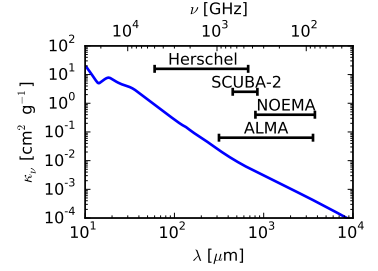
Figure 1.2: Milky Way dust absorption opacities per unit gas mass as a function of wavelength \lambda and frequency \nu in the infrared and sub-mm range, together with wavelength coverage of selected observational facilities. Dust opacities are taken from the model of Draine (2003) for R_V = 5.5 .
