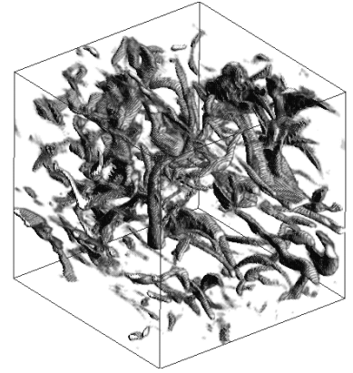
Figure 4.4: Volume rendering of the density field in a simulation of supersonic turbulence (Padoan & Nordlund, 1999). The surfaces shown are isosurfaces of density.
