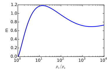
Figure A.3: Dimensionless mass m versus dimensionless density contrast \rho_c/\rho_s found by solving the isothermal Lane-Emden equation.
