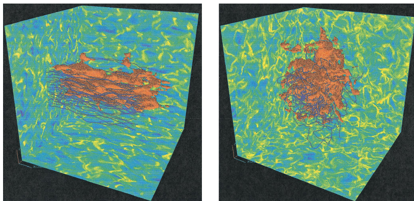
Figure 5.2: Simulations of Alfvénic (left) and sub-Alfvénic (right) turbulence. Colors on the cube surface are slices of the logarithm of density, blue lines are magnetic field lines, and red surfaces are isodensity surfaces for a passive contaminant added to the flow.
