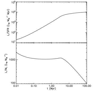
Figure 2.5: Bolometric luminosity versus time for stellar populations as a function of population age. The top panel shows the luminosity normalized by the star formation rate, while the bottom shows the luminosity normalized by the total stellar mass. Figure taken from Krumholz & Tan (2007).
