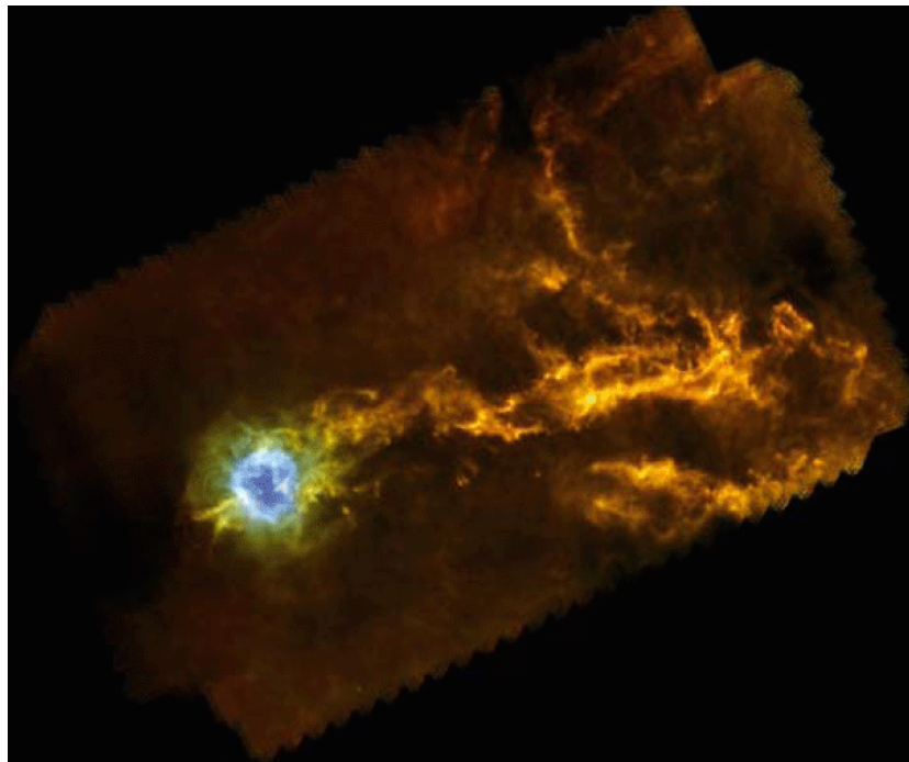
Figure 1.3: Three-color composite image of IC 5146 taken by the SPIRE and PACS instruments aboard Herschel . Red is SPIRE 500 \mu\text{m} , green is SPIRE 250 \mu\text{m} plus PACS 160 \mu\text{m} , and blue is PACS 70 \mu\text{m} . Image taken from Arzoumanian et al. (2011).
