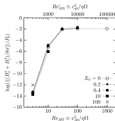
Figure 16.4: Results from a series of simulation of magneto-rotational instability with non-ideal MHD by Sano & Stone (2002). The y axis shows the mean Maxwell stress measured in the simulation once it reaches statistical steady state, normalized by the gas pressure. This is roughly the same as \alpha . Simulations are shown at a range of magnetic Reynolds numbers \text{Re}_M . Different values of the parameter X_0 correspond to different strengths of Hall diffusivity.
